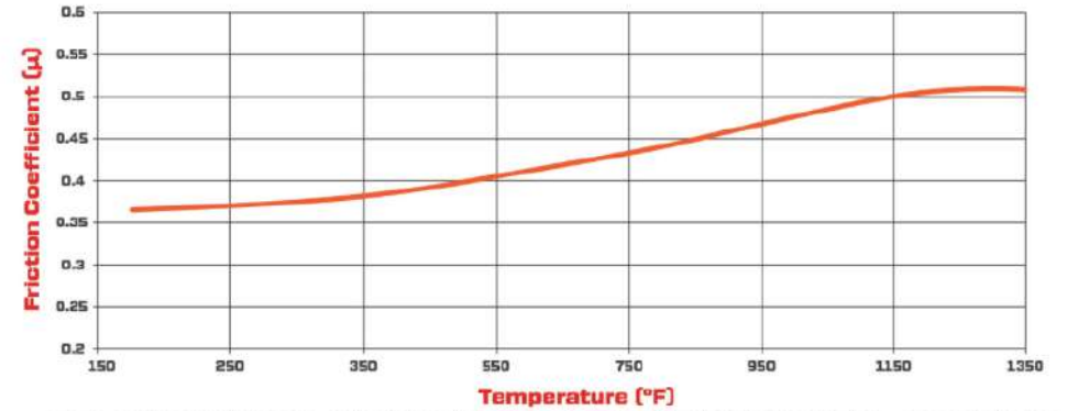
CM - Composite Metallic Friction Coefficient and Temperature Values
